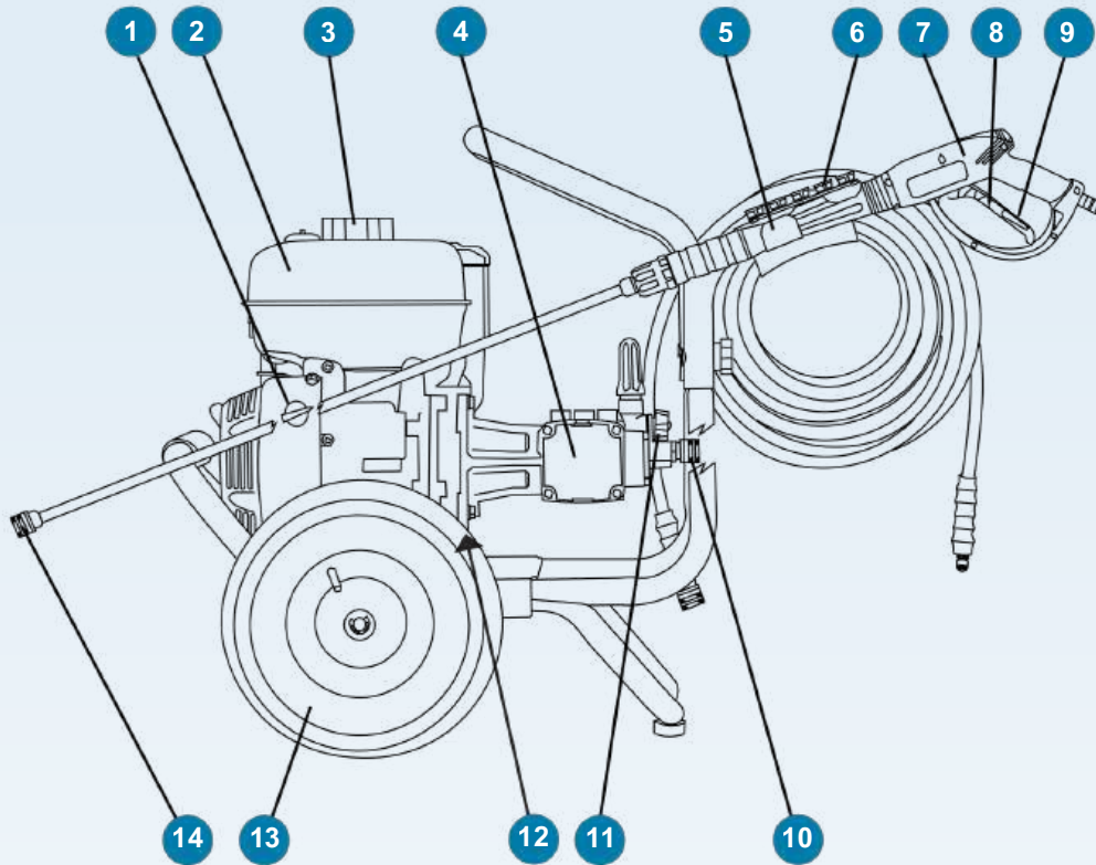
FRONT PERSPECTIVE
