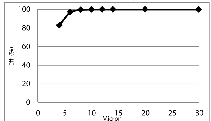
Average Filtration Efficiency (ISO 16889)
