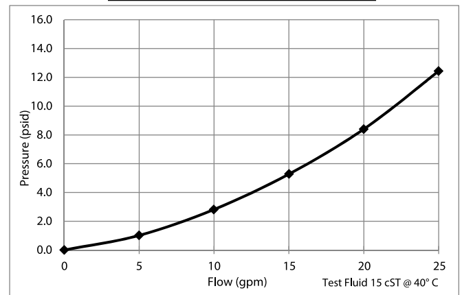
Flow Versus Pressure (ISO 3968)
