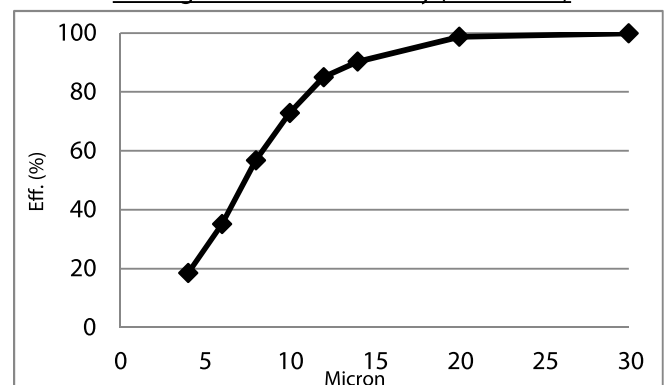
Average Filtration Efficiency (ISO 16889)
